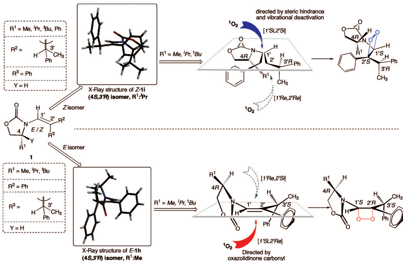
FIGURE 2. Preferred \pi -facial attack of ^1\text{O}_2 in Z- (top) and E-encarbamates (bottom). The conformations of the E/Z-encarbamates are based on the X-ray structures of Z- 1i and E- 1h .
